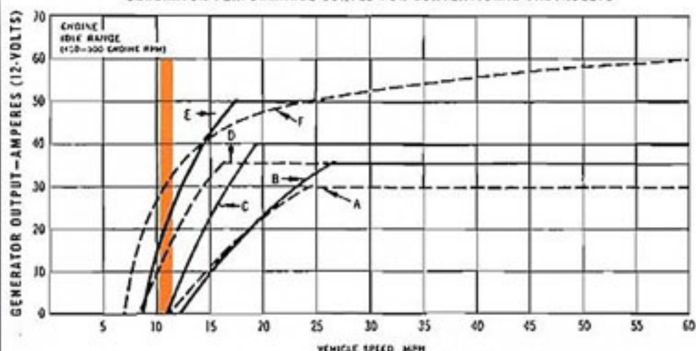
GENERATOR PERFORMANCE CURVES FOR CONVENTIONAL CHEVROLETS
