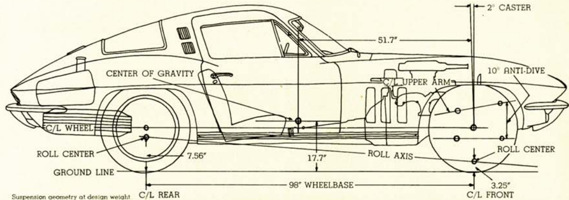
Suspension geometry at design weight
