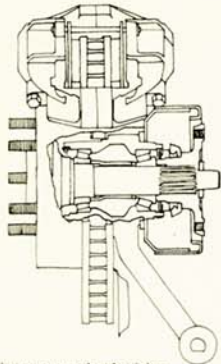
Rear brake linings on each side of disc
