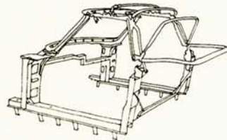
Soft top framework
