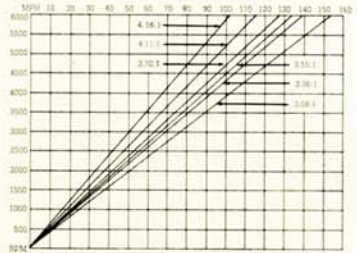
MILES PER HOUR PER 1000 ENGINE RPM IN FINAL DRIVE (Figures are estimated with no allowance for slippage or tire expansion)
