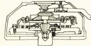
Clutch cutaway
