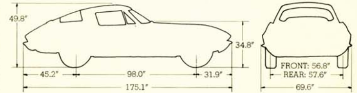
External dimensions, Sport Coupe
