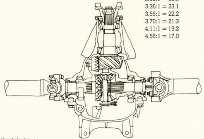
Differential cutaway
