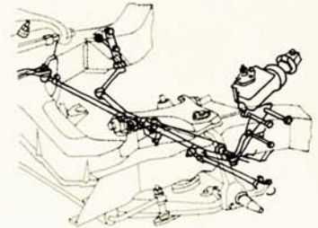
Steering system
