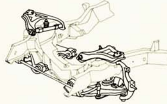
Front suspension
