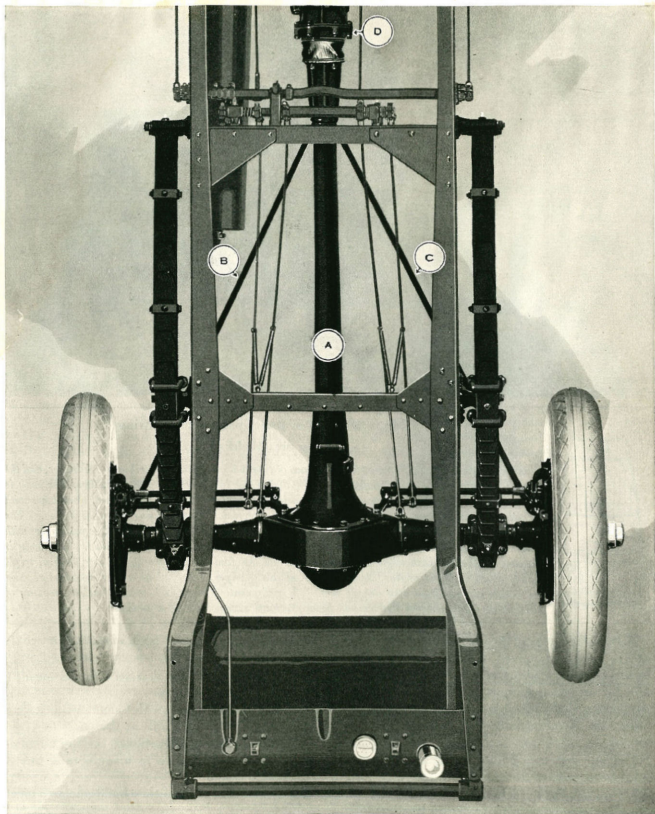
The McLaughlin-Buick torque tube drive
