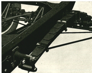
The McLaughlin-Buick cantilever rear springs.
