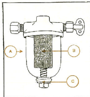
The operation of the gasoline filter or strainer is shown in this diagram. Point (A) indicates the glass container from which the gasoline passes through the screen (B), leaving all sediment in the glass. The glass may be easily removed and cleaned by unscrewing the nut (C). After a few thousand miles driving, the efficiency of this filter will be clearly demonstrated by the amount of dirt found in the glass.
