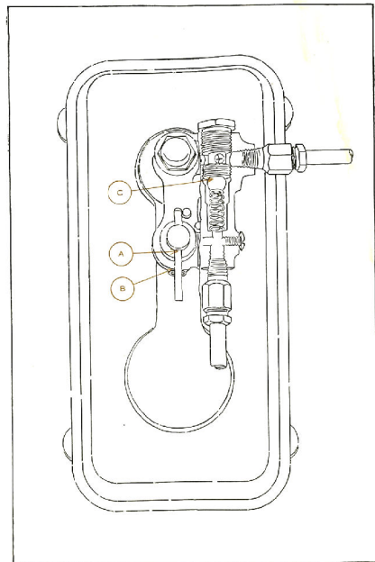
Turning the handle (A) permits oils to flow out at (B) if the oil filter is working. If the oil does not run out freely at (B), then the filter is not working properly. In this case the ball check valve (C) is forced down by the pressure of the oil, and oil flows to the outlet pipe without going through the filter, thus insuring lubrication of the engine under all conditions.
