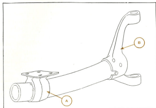
In this type of front axle the spring seats (A) and the yoke ends (B) are brazed and riveted on, making a less dependable axle than that used by McLaughlin-Buick, which is drop-forged in one piece, with no riveted or brazed parts.
