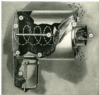
Diagram showing how the McLaughlin-Buick air cleaner presents dust from entering the carburetor.
