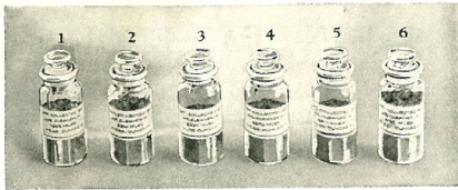
The efficiency of the McLaughlin Buick air cleaner is strikingly indicated by these bottles, which contain dirt collected from McLaughlin-Buick test cars by the air cleaner. The bottle on the left shows the amount of dirt collected in 7,593 miles driving—2.15 ounces. Bottle No. 2—6,941 miles—2.64 ounces. Bottle No. 3—6,290 miles—1.68 ounces. Bottle No. 4—3,505 miles—2.29 ounces. Bottle No. 5—4,317 miles—1.35 ounces. Bottle No. 6—8,136 miles—3.01 ounces.
