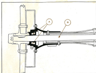
is the semi-floating axle. In this type the bearing (A) is mounted directly on the axle shaft (B) with the result that the shaft must carry the weight of the car in addition to turning the wheel. If the shaft breaks the wheel comes off.
