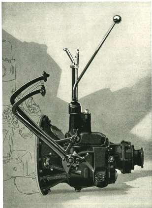
The McLaughlin-Buick transmission.
