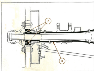
The McLaughlin-Buick floating rear axle. In this type the bearing (A) is mounted on the rear housing (B). The weight of the car is on the housing, not on the shaft. If the shaft break the wheel does not come off, and the car may be towed.
