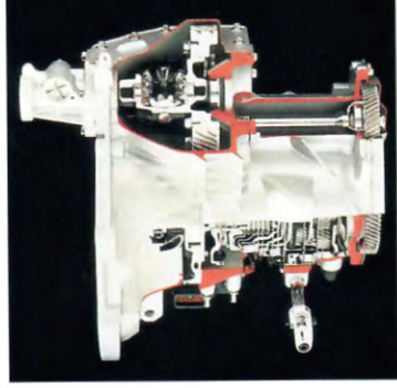
An electronically controlled four-speed overdrive transaxle offers quick acceleration, improved fuel efficiency and quiet cruising.
