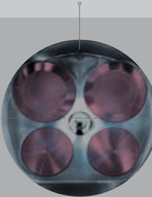
Four valves per cylinder
