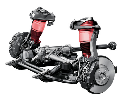
Audi adaptive air suspension (optional on Prestige models)
