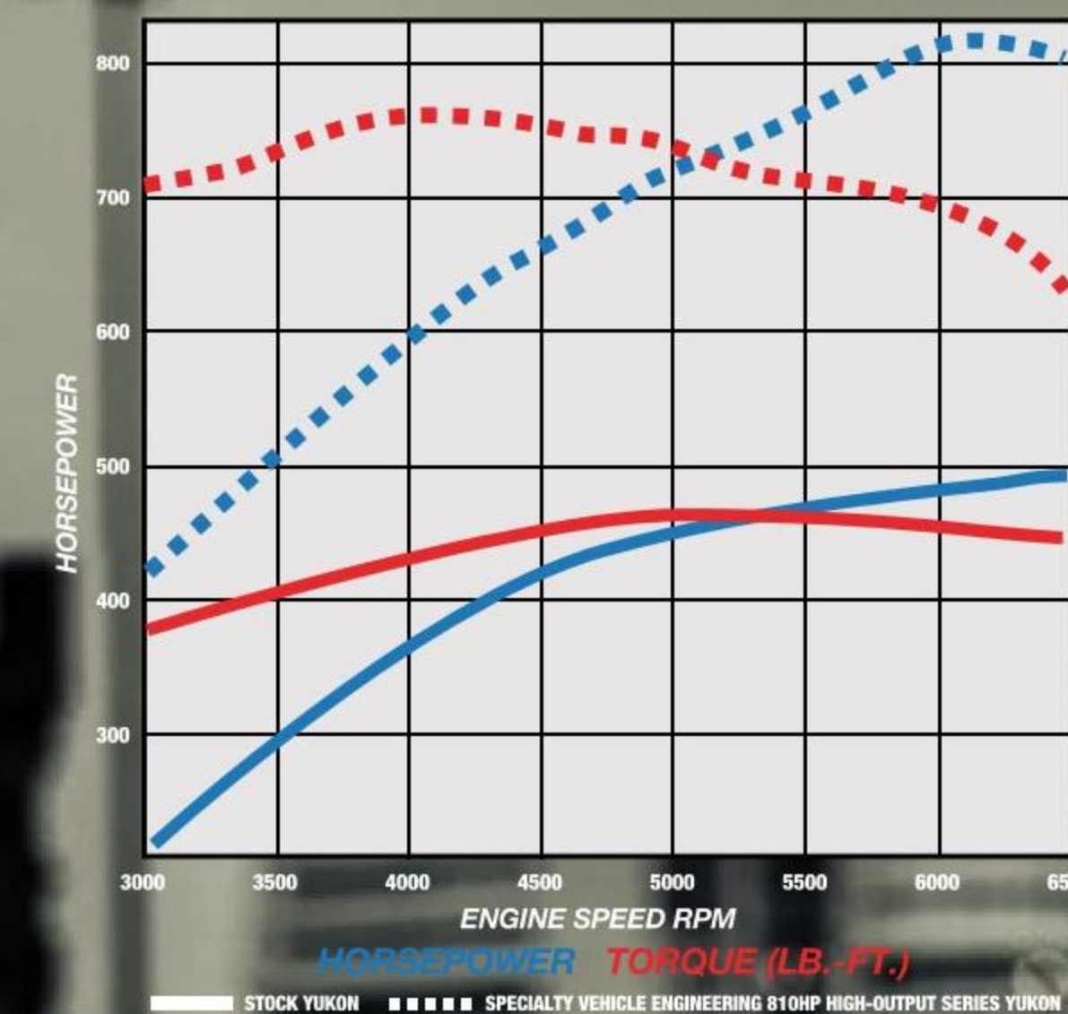
2019 810HP 6.8L HIGH/OUTPUT SERIES YUKON FLYWHEEL HORSEPOWER and TORQUE (lb.-ft.)
