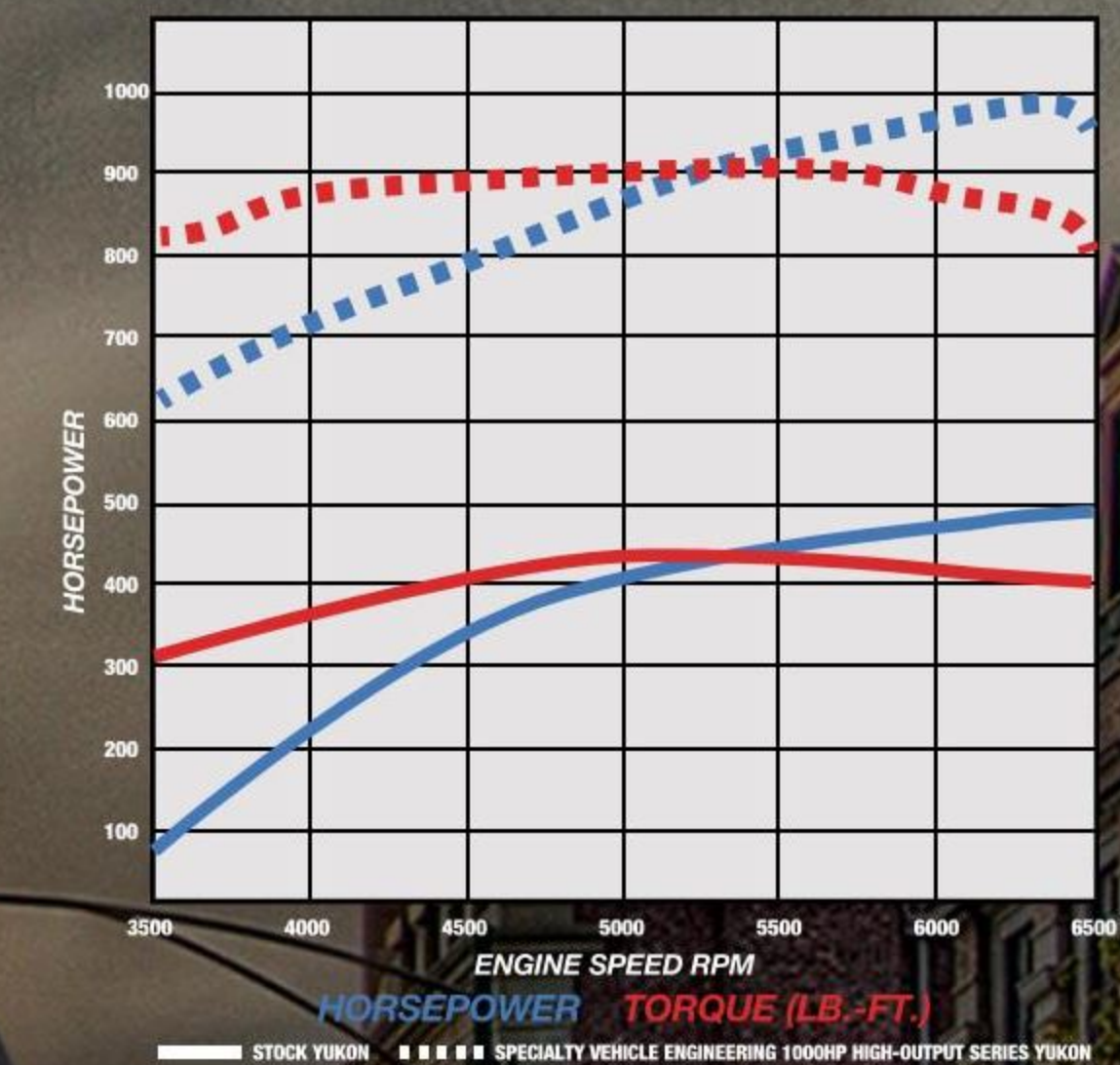
2019 1000HP 6.8L HIGH/OUTPUT SERIES YUKON FLYWHEEL HORSEPOWER and TORQUE (lb.-ft.)
