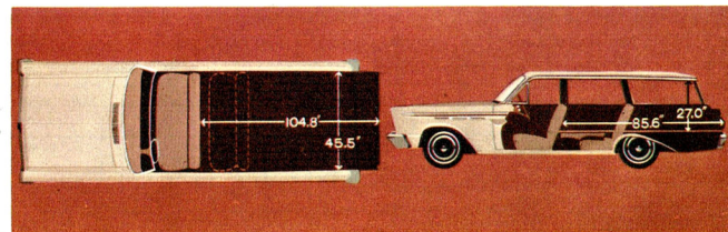
Comet station wagon interior dimensions.
