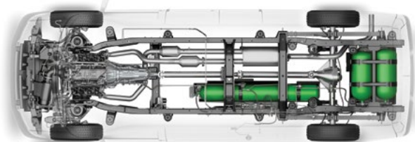
THREE-TANK SYSTEM
