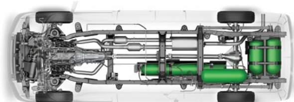
FOUR-TANK SYSTEM
