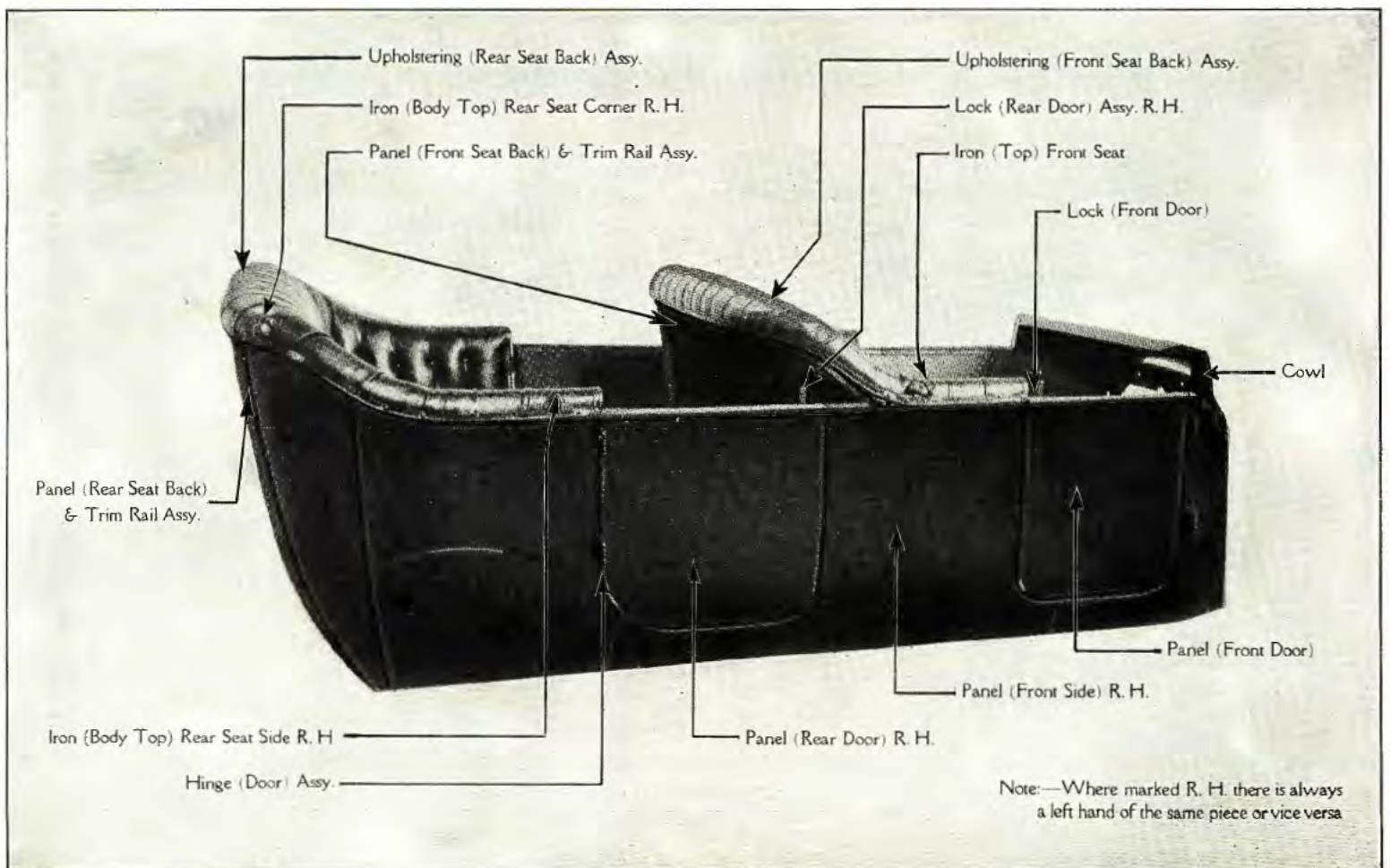
TOURING BODY
