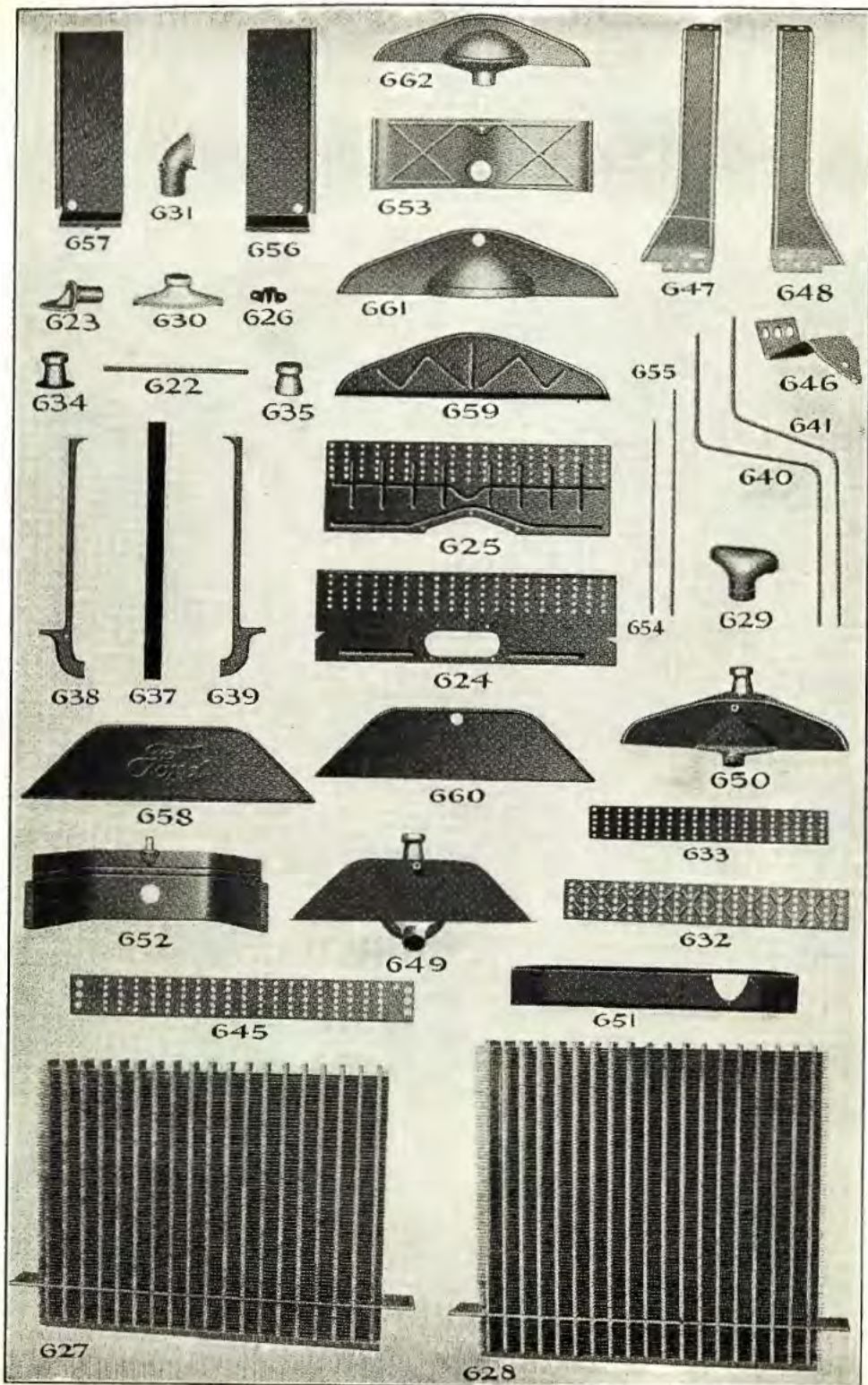
RADIATOR PARTS
