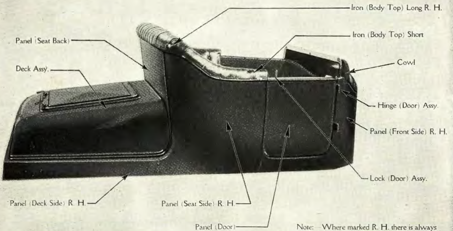
TORPEDO BODY
