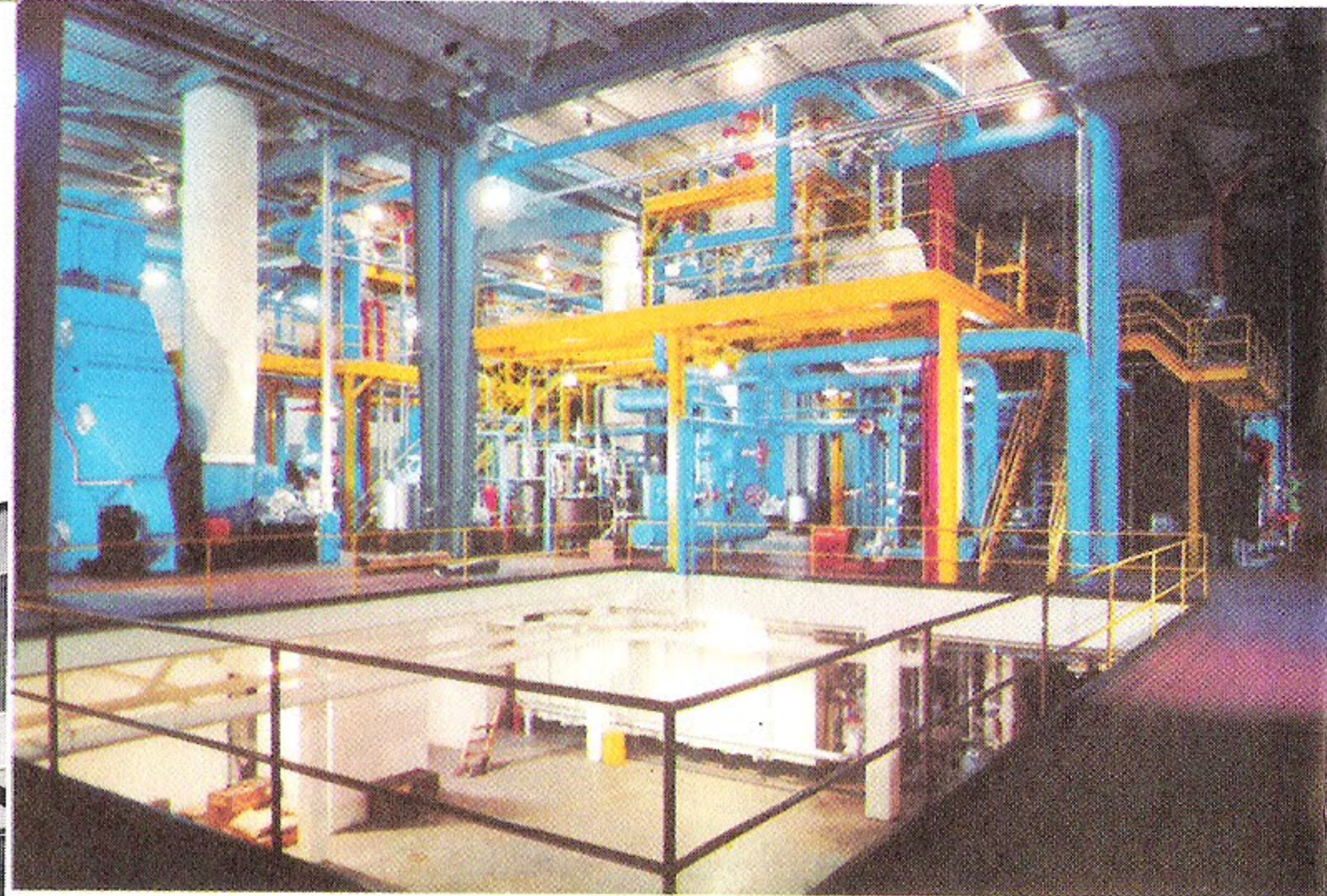
The Steam Plant has capacity of 440,000 pounds of steam every hour.
