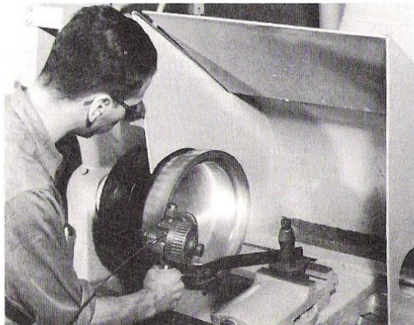
Application of sprayed molten metal to an experimental part.
