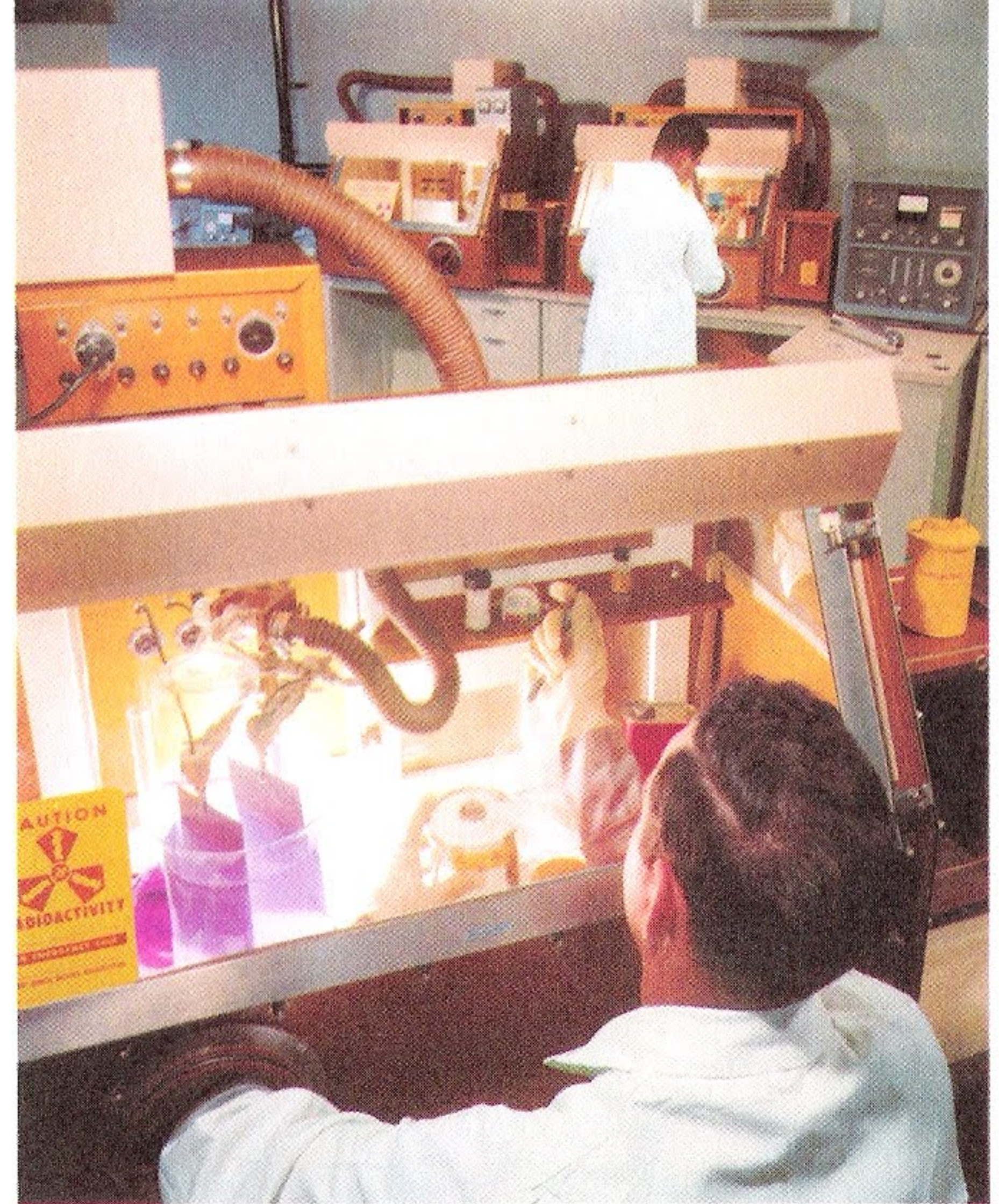
Radioactive isotopes are new tools in Research investigations. ★
