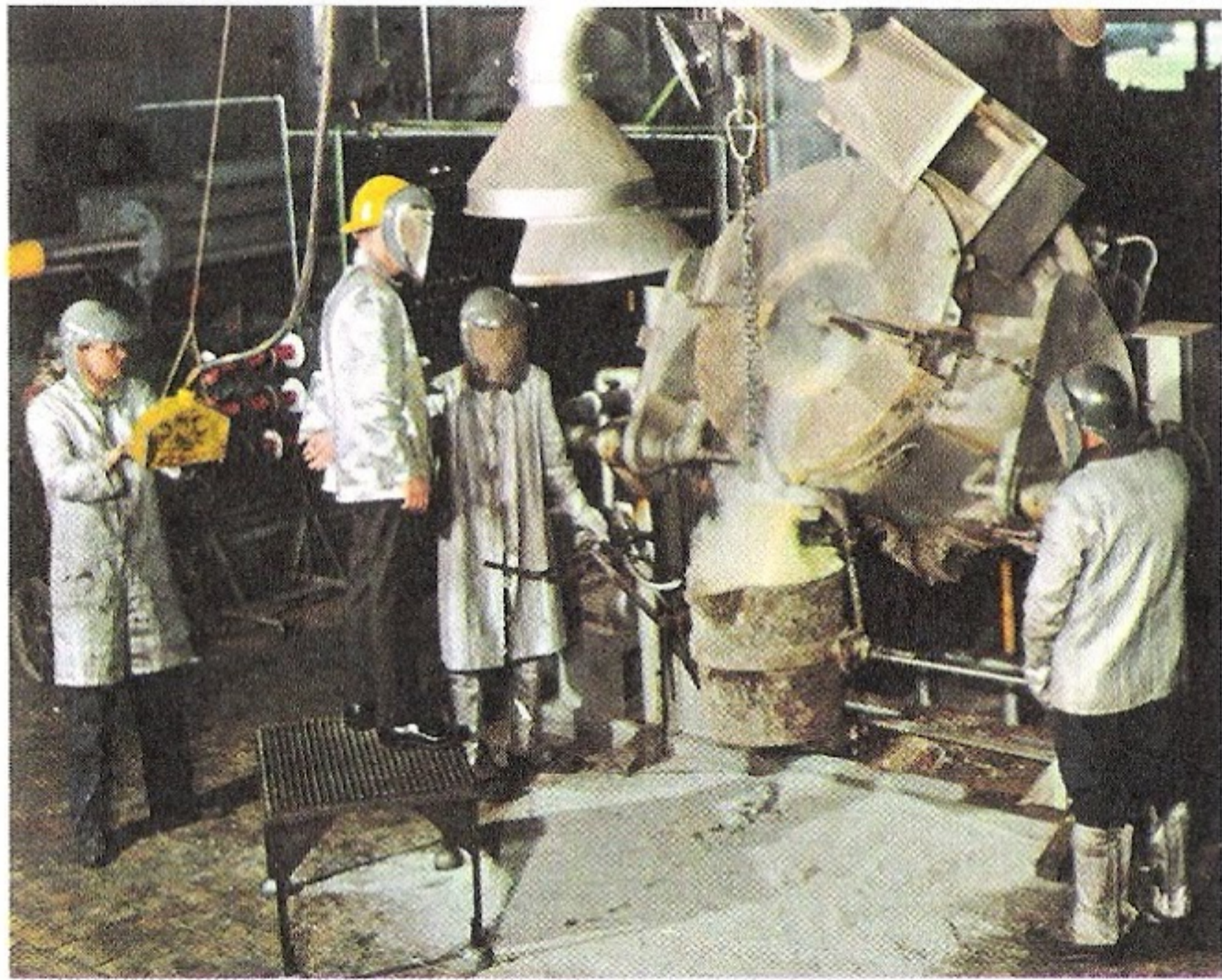
A complete metal casting facility is included to study casting techniques.
