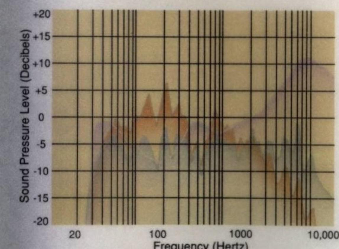
Frequency Response Prior To Equalization Equalizer Gain Frequency Response After Equalization
