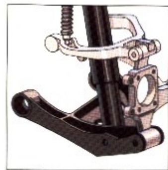
◀ The geometry of Short/Long Arm rear suspension allows for better contact between your tires and the road.
