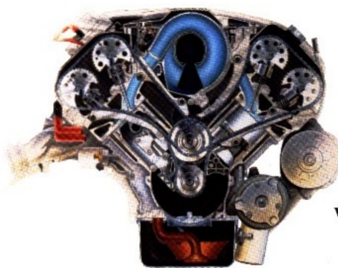
Three refined drive chains operate the Northstar V8's four camshafts. Design goals: no replacement or adjustments for 100,000 miles, and uncompromised quiet.
