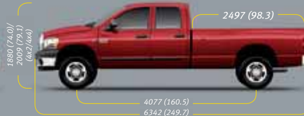
QUAD CAB – LONG BOX
