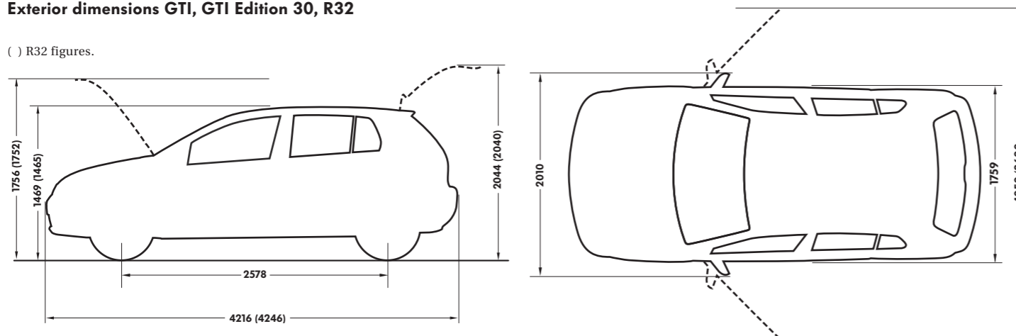
Exterior dimensions GTI, GTI Edition 30, R32
