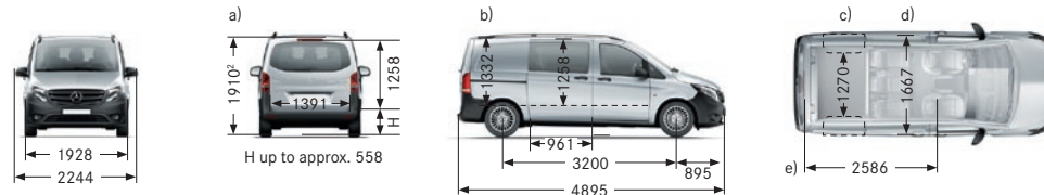
Compact crew van with 3200mm wheelbase
