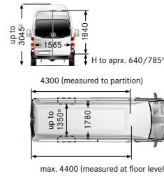
Long with 4325 mm wheelbase, super-high roof
