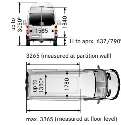
Medium with 3665 mm wheelbase, super-high roof
