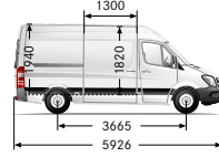
Medium with 3665 mm wheelbase, high roof
