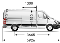
Medium with 3665 mm wheelbase, normal roof
