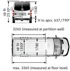
Medium with 3665 mm wheelbase, normal roof
