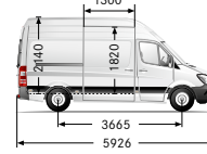
Medium with 3665 mm wheelbase, super-high roof
