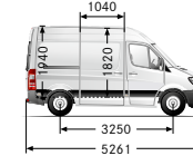
Short with 3250 mm wheelbase, high roof
