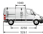
Short with 3250 mm wheelbase, normal roof
