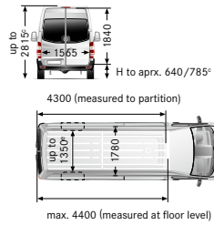
Long with 4325 mm wheelbase, super-high roof
