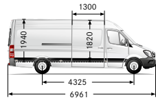
Long with 4325 mm wheelbase, normal roof
