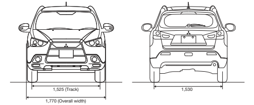
Ground Clearance Petrol – 195mm / Diesel – 180mm
