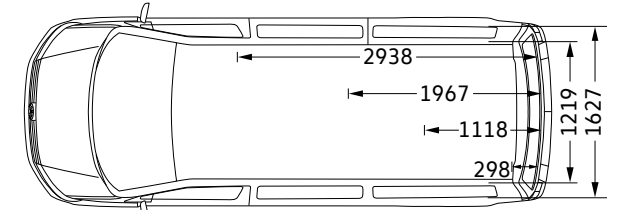
Vehicle dimensions shown in mm.
