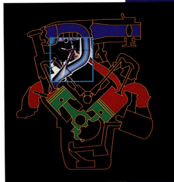
Smooth power is supplied by Grand Marquis' 5.0 litre V-8. The engine features sequential multi-port electronic fuel injection to enhance performance and fuel economy.
